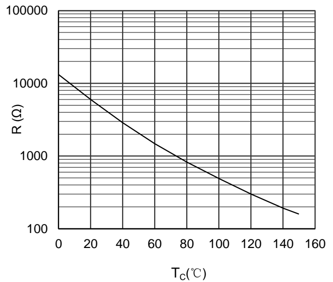
Figure 14. NTC Characteristics
