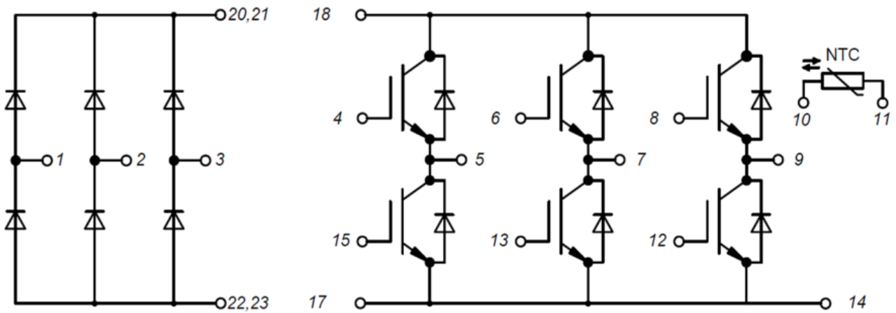
Figure 15. Circuit Diagram
