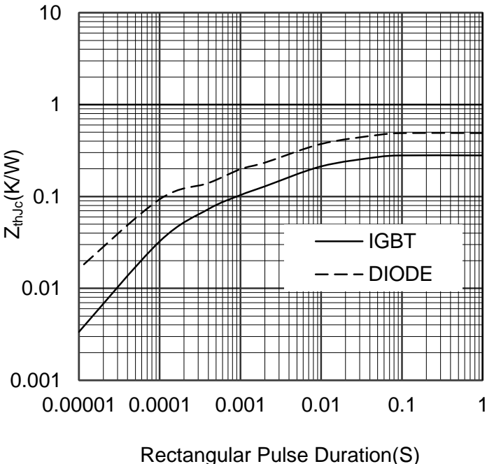
Figure 10. Transient Thermal Impedance of Diode and IGBT
